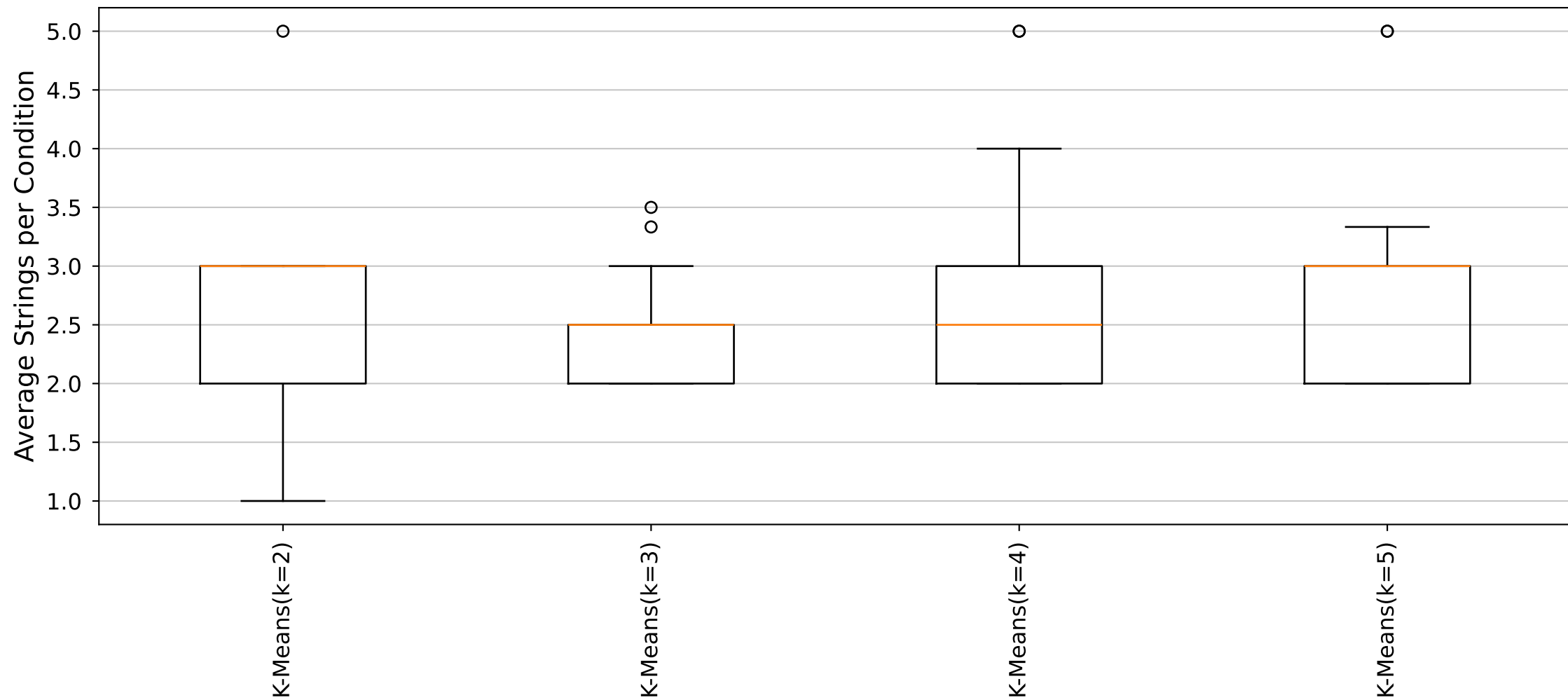
YARA Rules Average Strings per Condition Distribution (Cluster40_Size5 dataset)
